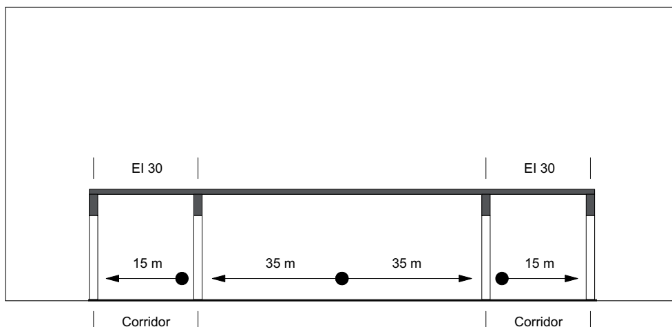
Escape route length with one or more exits with additionally protected corridors (EI 30)
